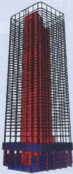
Figure 2: 3D FEA model of structure.
