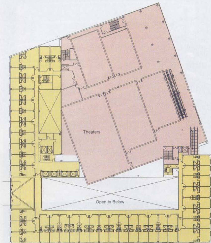
4TH FLOOR - TYPICAL THEATER LEVEL
